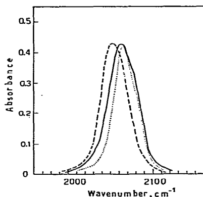
Fig. 4. Infrared absorption of 0.1\text{ M C}_2\text{H}_4\text{Cl}_2 solutions of tetrahedral isothiocyanates in the 2000\text{--}2100\text{ cm}^{-1} range:
