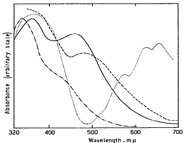
Fig. 1. Reflectance spectra of [\text{Co}(\text{PEt}_3)_2(\text{NCS})_2] (—), [\text{Co}(\text{diarsine})_2(\text{CNS})_2] (-.-.-), [\text{Co}(\text{CNCH}_3)_4][\text{CdBr}_4] (---), [\text{Co}(\text{PCy}_3)_2(\text{NCS})_2] (.....).
